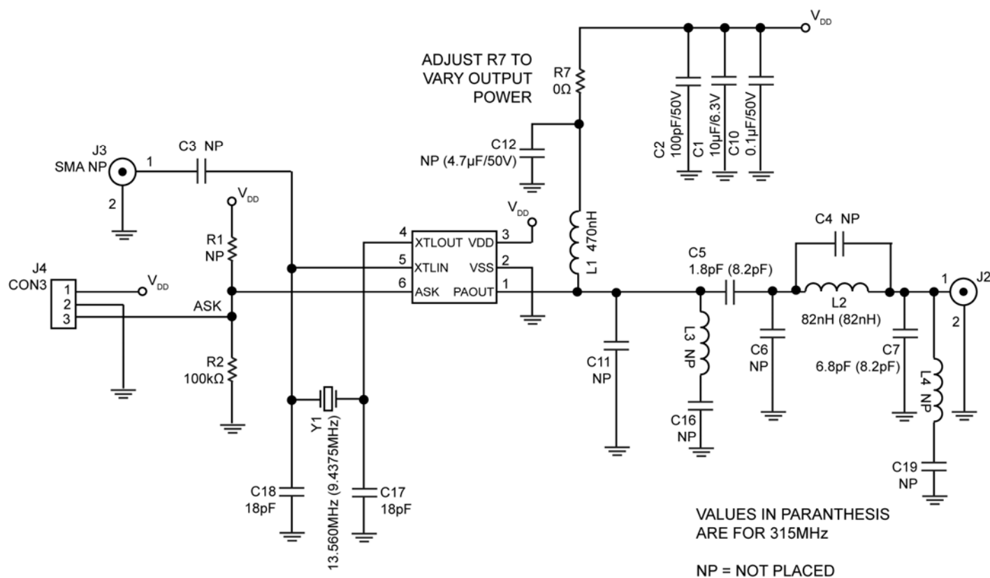
Figure 2. MICRF113 Test Circuit with 50Ω Output
