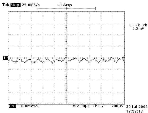
Figure 4: Output Ripple & Noise ( V_{in}=5.5V , V_{out}=0.59V/10A , Environment Temp= 25^{\circ}C )
