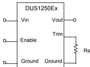
Figure 56: Trimming Output Voltage
