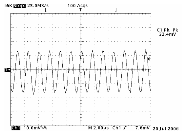
Figure 12: Output Ripple & Noise ( V_{in}=13.2V , V_{out}=5V/10A , Environment Temp.=25°C)
