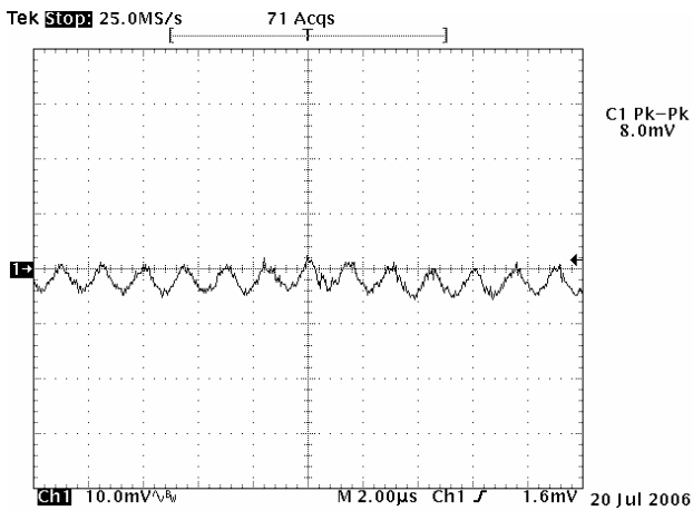
Figure 9: Output Ripple & Noise ( V_{in}=12V , V_{out}=1.5V/10A , Environment Temp.=25°C)
