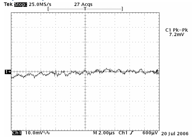
Figure 8: Output Ripple & Noise ( V_{in}=12V , V_{out}=0.59V/10A , Environment Temp.=25°C)
