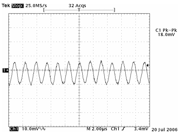
Figure 11: Output Ripple & Noise ( V_{in}=12V , V_{out}=3.3V/10A , Environment Temp.=25°C)
