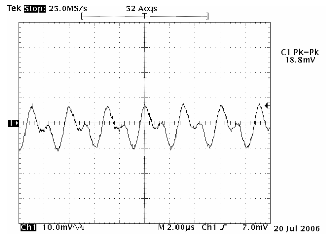
Figure 10: Output Ripple & Noise ( V_{in}=13.2V , V_{out}=2.5V/10A , Environment Temp.=25°C)
