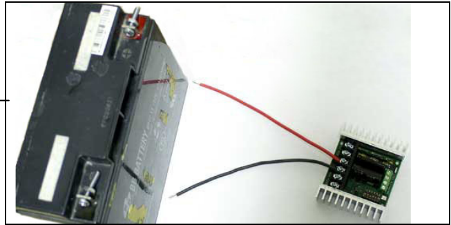
The battery connects to terminals B+ and B-
