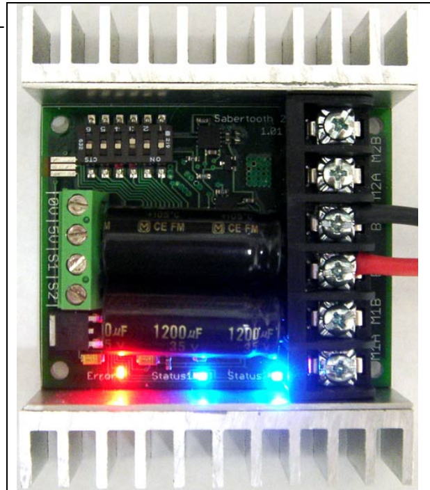
All Status LEDs on
