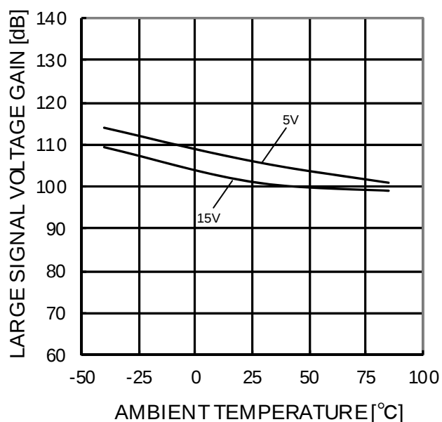
Figure 22. Large Signal Voltage Gain - Ambient Temperature ( R_L=2k\Omega )
