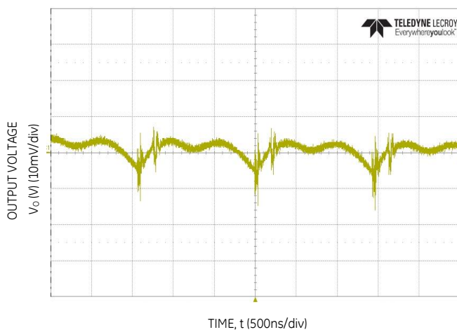
Figure 9. Typical output ripple and noise ( C_o=2 \times 47\mu F ceramic, V_{in} = 12V , I_o = I_{o,max} ).
