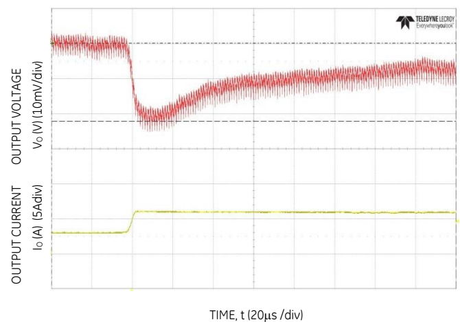
Figure 10. Transient Response to Dynamic Load Change from 50% to 100% at 12V in , C_{out}=3 \times 47\mu F + 2 \times 330\mu F , C_{Tune}=5600pF , R_{Tune}=300\Omega
