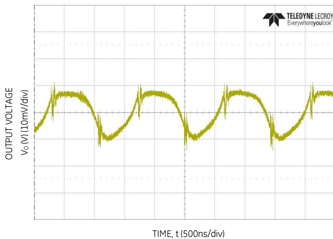
Figure 33. Typical output ripple and noise ( C_o=2 \times 47\mu F ceramic, V_{IN} = 12V , I_o = I_{o,max} ).
