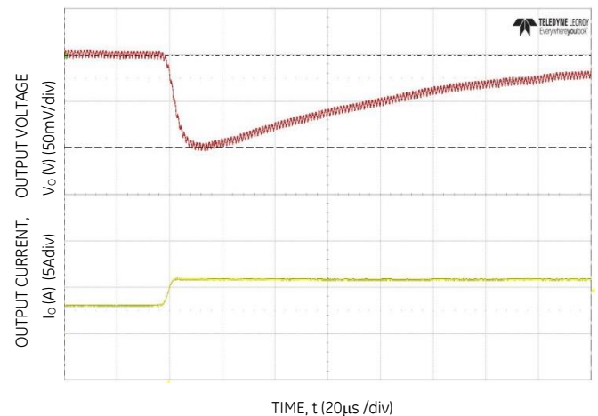
Figure 34. Transient Response to Dynamic Load Change from 50% to 100% at 12Vin, C_{out}=5 \times 47\mu F , C_{Tune}=1800pF , R_{Tune}=300\Omega
