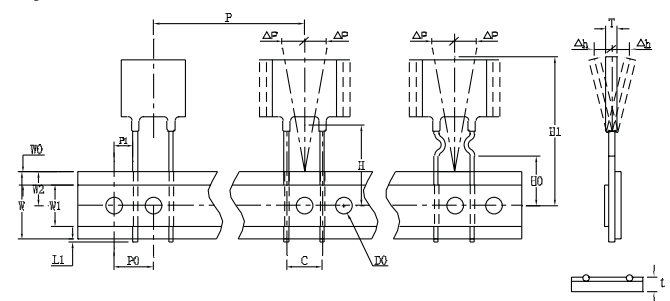
Style 2 - PTR016V1200-PTR016V1500
