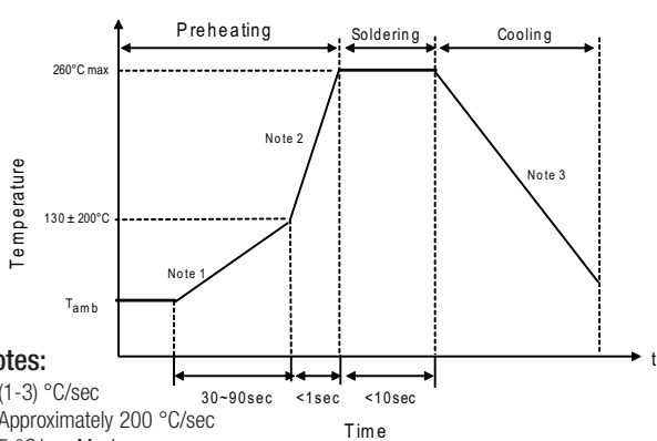
Recommended Wave Solder Profile
