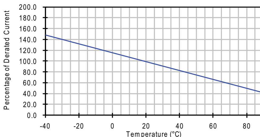
Thermal Derating Curve
