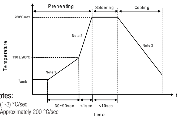
Recommended Wave Solder Profile
