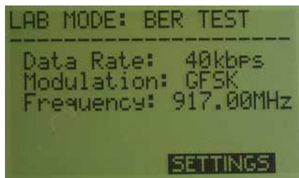
Figure 47. Runtime Screen
