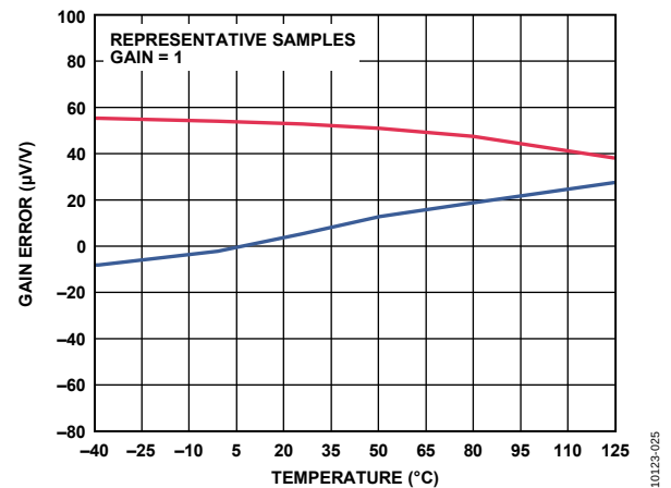
Figure 26. Gain vs. Temperature (G = 1)
