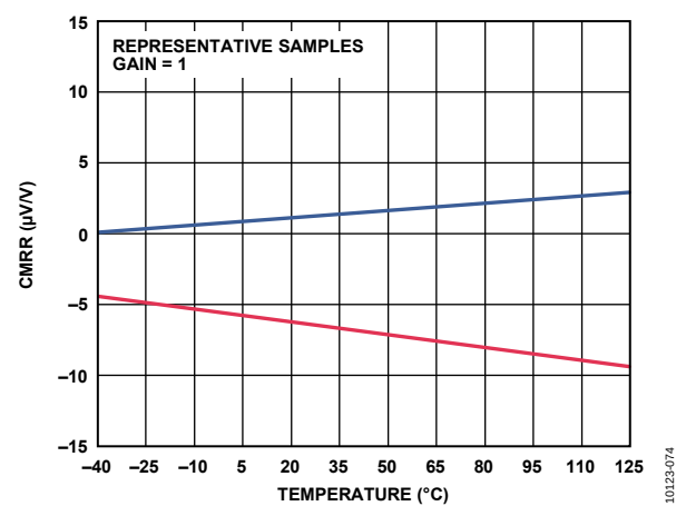
Figure 27. CMRR vs. Temperature (G = 1)
