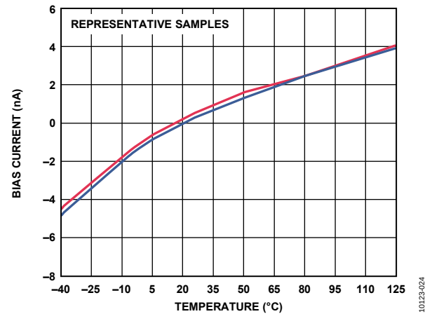
Figure 25. Input Bias Current vs. Temperature
