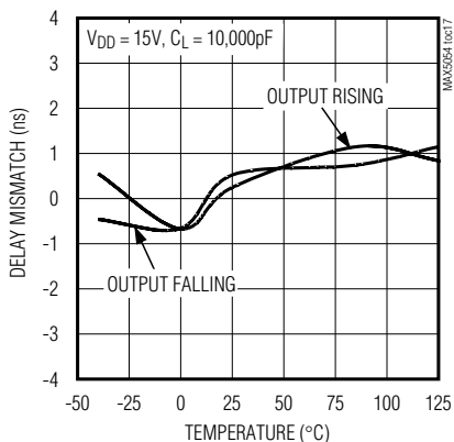
DELAY MISMATCH BETWEEN 2 CHANNELS vs. TEMPERATURE
