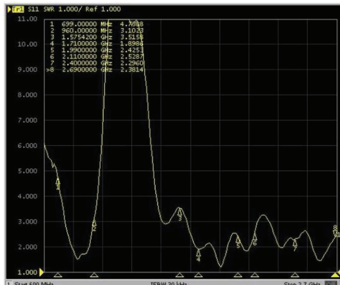
LTE S11 (VSWR)
