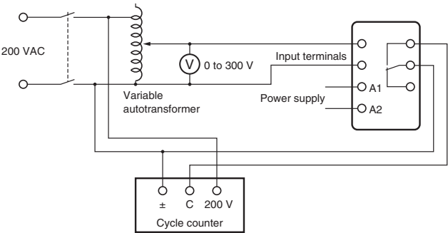
Connection Diagram
