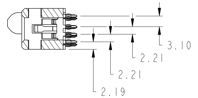
SECTION Z-Z
