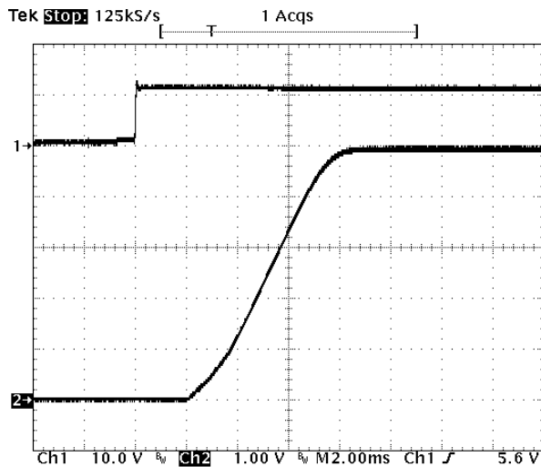
Fig-5.0V-4: Turn-on transient for Vout=5.0V with application of Vin at full rated load current (resistive) and 47 \mu Fx2 external capacitance at Vin=12.0V.
