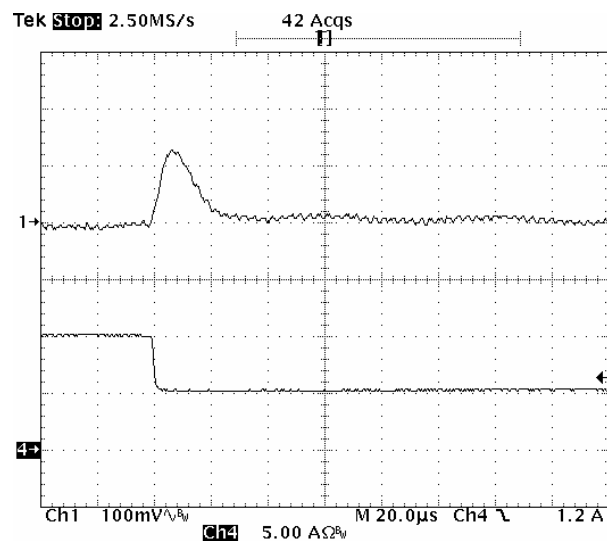
Fig-1.8V-7: Output voltage response for V_{out}=1.8V to positive load current step-change from 10A to 5A with slew rate of -5A/\mu s at V_{in}=12.0V . C_o=47\mu F \times 2 ceramic.
