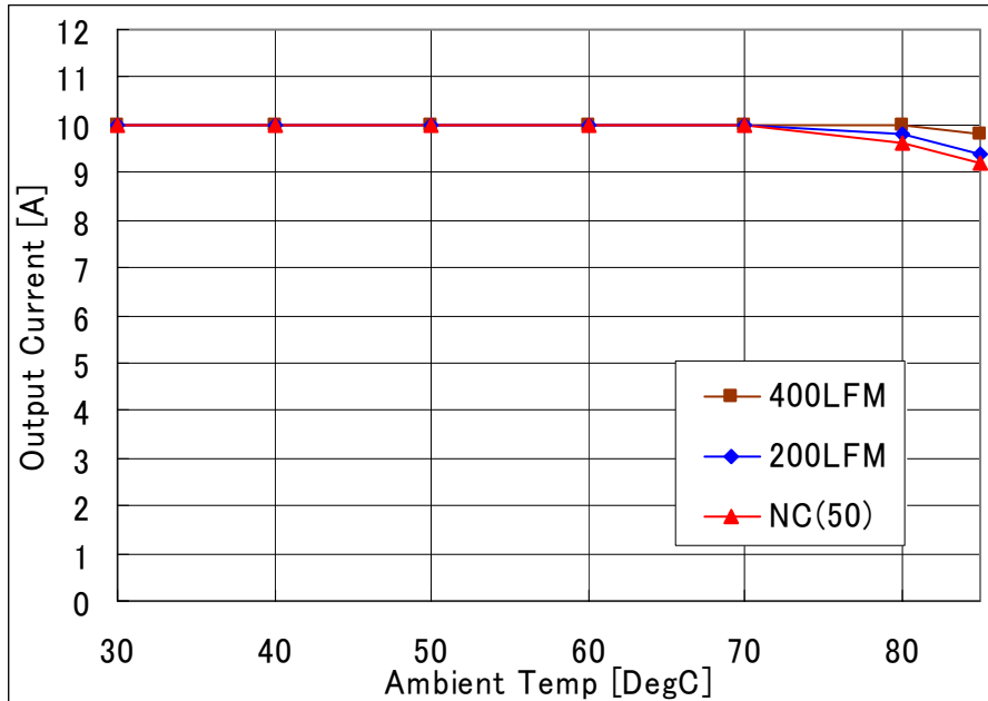
Fig-1.8V-1: Available load current vs. ambient temperature and airflow rates for V_{out}=1.8V with V_{in}=12.0V . Maximum component temperature \leq 120^{\circ}C
