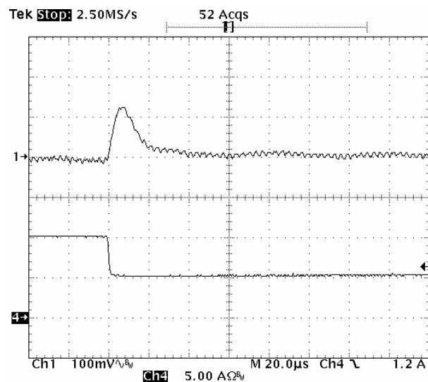
Fig-2.0V-7: Output voltage response for V_{out}=2.0V to positive load current step-change from 10A to 5A with slew rate of -5A/\mu s at V_{in}=12.0V . C_o=47\mu F \times 2 ceramic.
