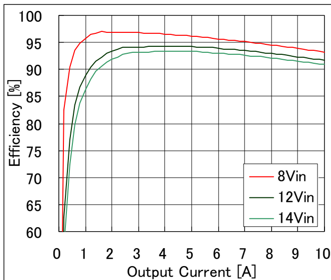
Fig-5.0V-2: Efficiency vs. load current and input voltage for V_{out}=5.0V . Airflow rate=200 LFM (1.0m/s) and T_a=25^{\circ}C .
