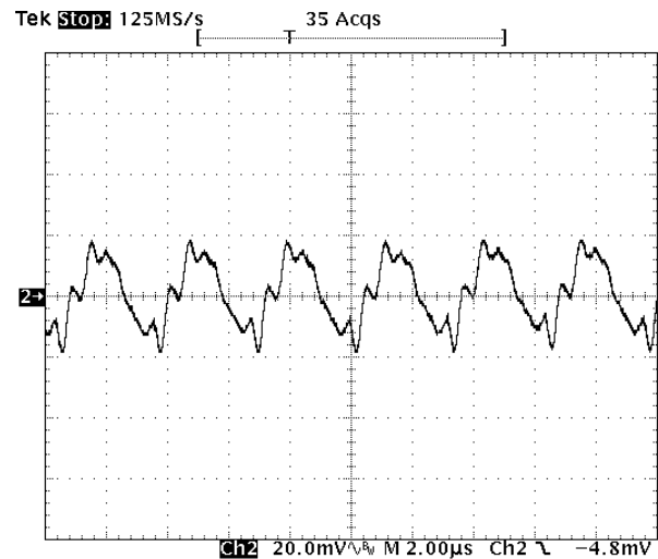
Fig-5.0V-5: Output voltage ripple (20mV/div.) for Vout=5.0V at full rated load current into a resistive load with external capacitance 47 \mu Fx2 ceramic + 1 \mu F ceramic at Vin=12.0V.
