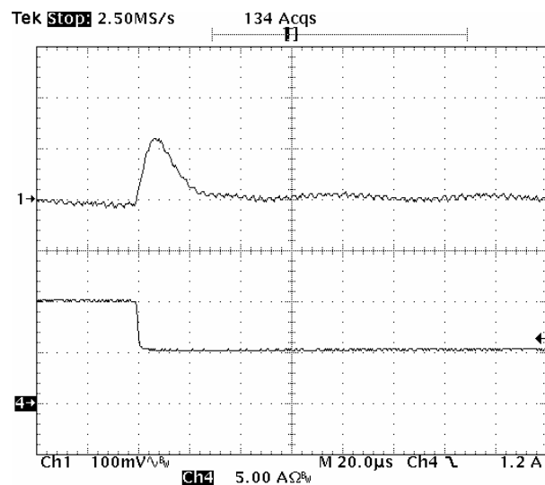
Fig-1.5V-7: Output voltage response for V_{out}=1.5V to positive load current step-change from 10A to 5A with slew rate of -5A/\mu s at V_{in}=12.0V . C_o=47\mu F \times 2 ceramic.
