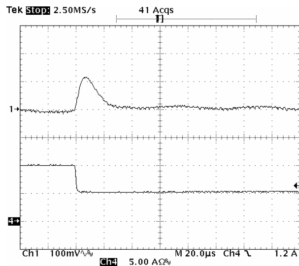
Fig-1.2V-7: Output voltage response for V_{out}=1.2V to positive load current step-change from 10A to 5A with slew rate of -5A/\mu s at V_{in}=12.0V . C_o=47\mu F \times 2 ceramic.
