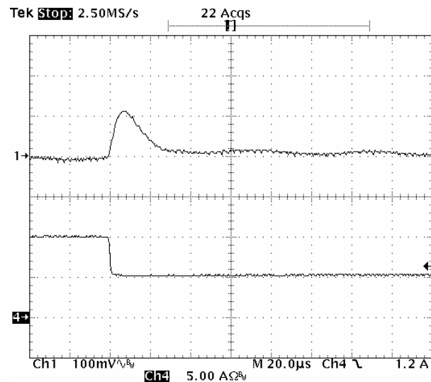
Fig-1.0V-7: Output voltage response for V_{out}=1.0V to positive load current step-change from 10A to 5A with slew rate of -5A/\mu s at V_{in}=12.0V . C_o=47\mu F \times 2 ceramic.
