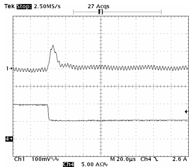
Fig-5.0V-7: Output voltage response for Vout=5.0V to positive load current step-change from 10A to 5A with slew rate of -5A/ \mu s at Vin=12.0V. Co=47 \mu Fx2 ceramic.
