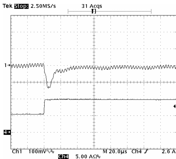
Fig-5.0V-6: Output voltage response for Vout=5.0V to positive load current step-change from 5A to 10A with slew rate of 5A/ \mu s at Vin=12.0V. Co=47 \mu Fx2 ceramic.
