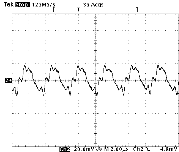
Fig-5.0V-5: Output voltage ripple (20mV/div.) for V_{out}=5.0V at full rated load current into a resistive load with external capacitance 47\mu F \times 2 ceramic + 1\mu F ceramic at V_{in}=12.0V .
