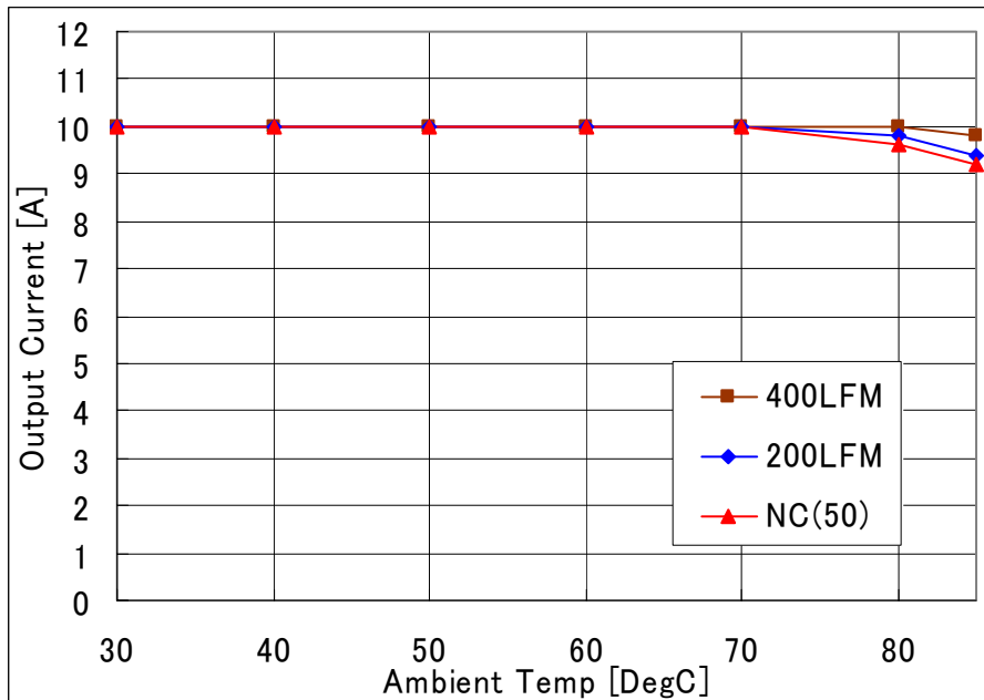
Fig-1.5V-1: Available load current vs. ambient temperature and airflow rates for V_{out}=1.5V with V_{in}=12.0V . Maximum component temperature \leq 120^{\circ}C
