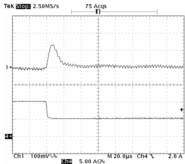
Fig-3.3V-7: Output voltage response for V_{out}=3.3V to positive load current step-change from 10A to 5A with slew rate of -5A/\mu s at V_{in}=12.0V . C_o=47\mu F \times 2 ceramic.
