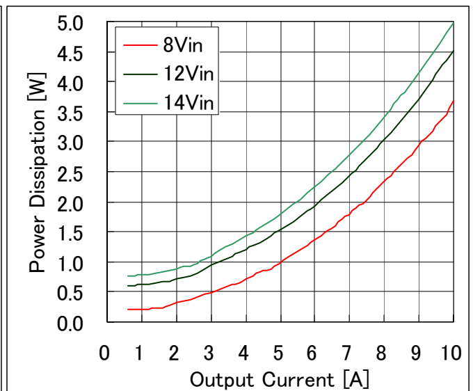
Fig-5.0V-3: Power dissipation vs. load current and input voltage for V_{out}=5.0V . Airflow rate=200 LFM (1.0m/s) and T_a=25^{\circ}C .
