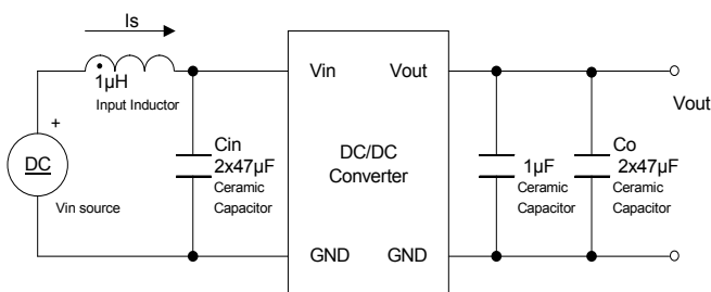
Fig. D: Test setup for measuring output voltage ripple
