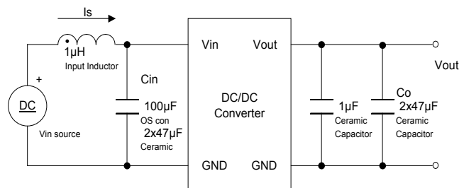
Fig. E: Test setup for measuring input reflected ripple current
