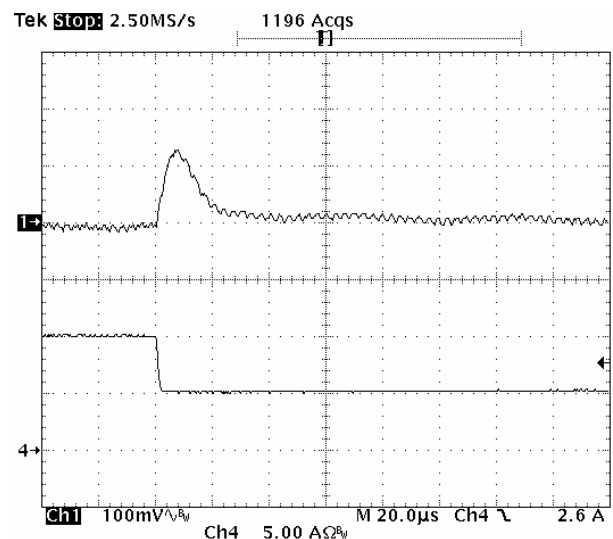
Fig-2.5V-7: Output voltage response for V_{out}=2.5V to positive load current step-change from 10A to 5A with slew rate of -5A/\mu s at V_{in}=12.0V . C_o=47\mu F \times 2 ceramic.
