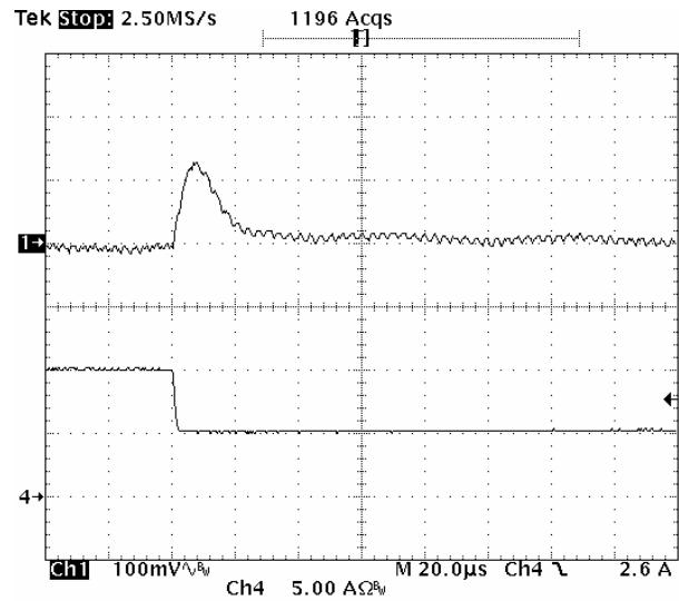
Fig-2.5V-7: Output voltage response for V_{out}=2.5V to positive load current step-change from 10A to 5A with slew rate of -5A/\mu s at V_{in}=12.0V . C_o=47\mu F \times 2 ceramic.
