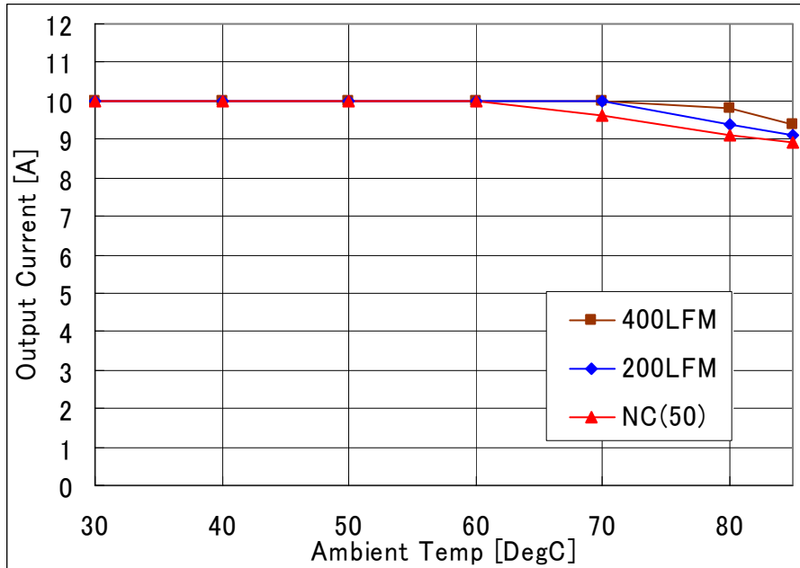
Fig-2.5V-1: Available load current vs. ambient temperature and airflow rates for Vout=2.5V with Vin=12.0V. Maximum component temperature \leq 120°C
