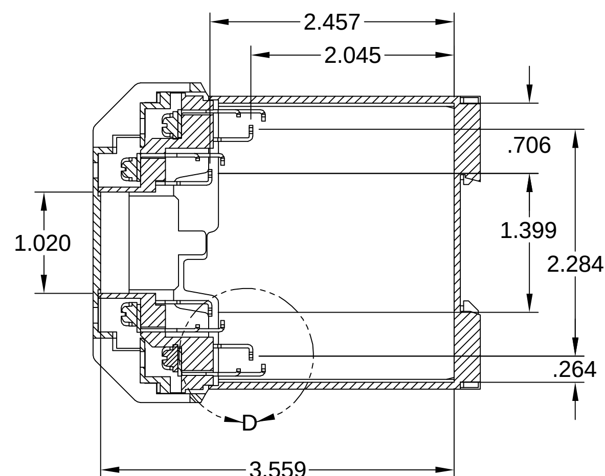
SECTION B-B
