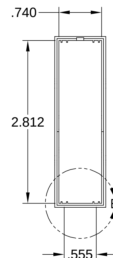
SECTION C-C
