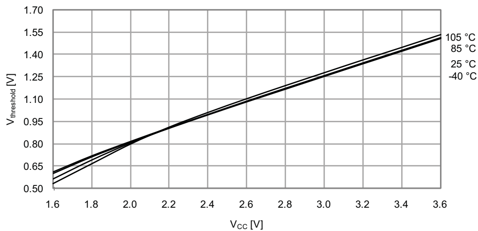
Figure 36-28. I/O Pin Input Threshold Voltage vs. V_{CC}
