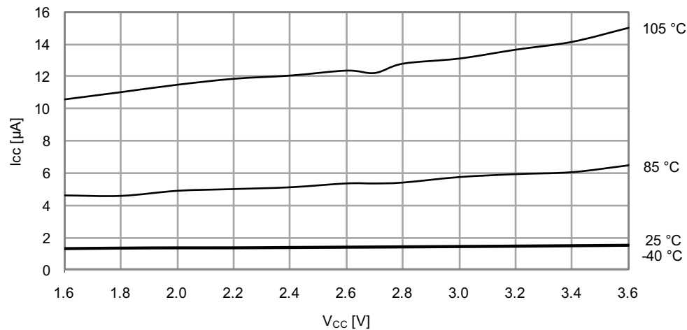
Figure 36-16.Power-down Mode Supply Current vs. V_{CC} Watchdog and sampled BOD enabled
