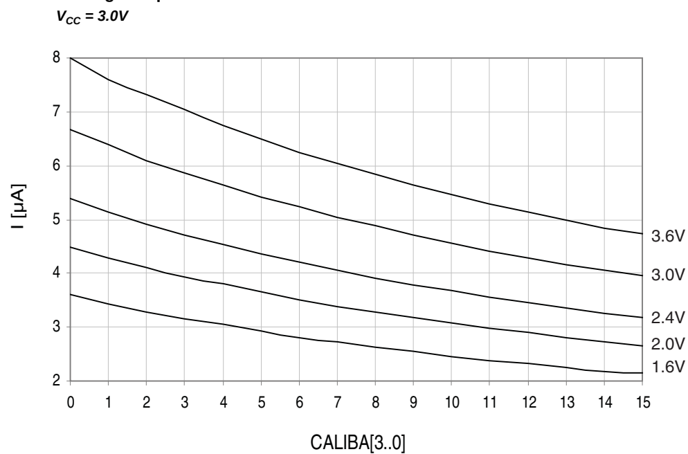
Figure 36-43. Analog Comparator Current Source vs. Calibration Value
