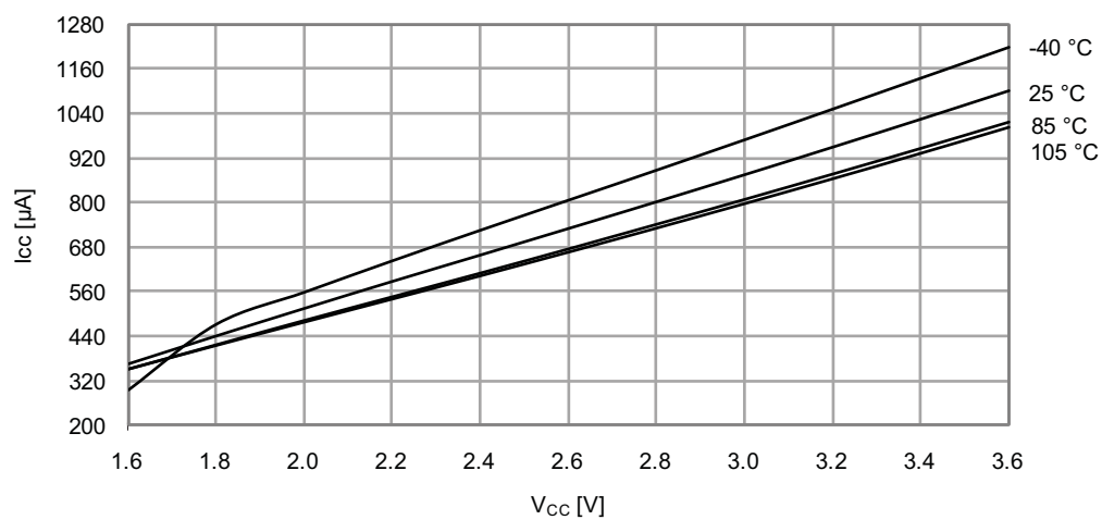
Figure 36-4. Active Mode Supply Current vs. V_{CC}
