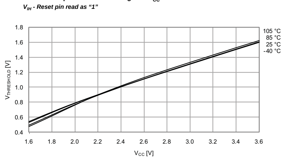
Figure 36-52. Reset Pin Input Threshold Voltage vs. V_{CC}
