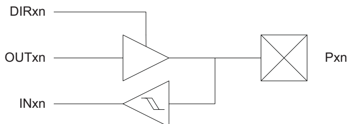
Figure 15-1. I/O Configuration - Totem-pole
