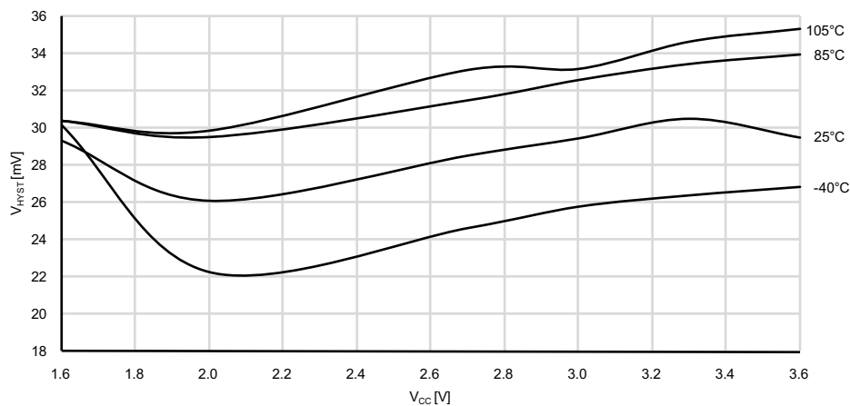
Figure 36-42. Analog Comparator Hysteresis vs. V_{CC} Large hysteresis
