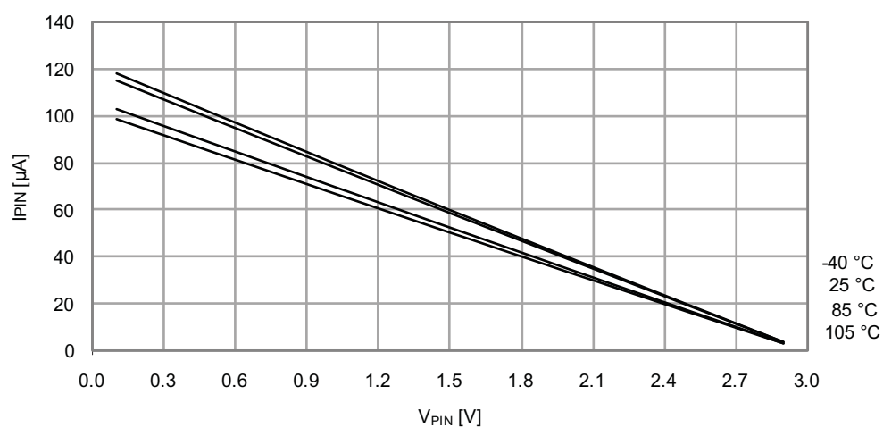
Figure 36-19. I/O Pin Pull-up Resistor Current vs. Input Voltage
