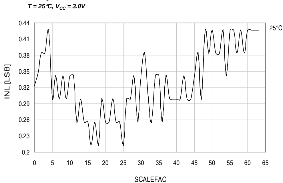
Figure 36-44. Voltage Scaler INL vs. SCALEFAC
