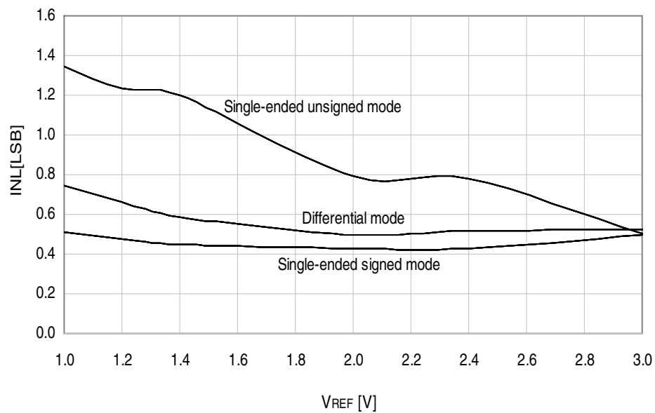
Figure 36-30. INL Error vs. External V_{REF}
