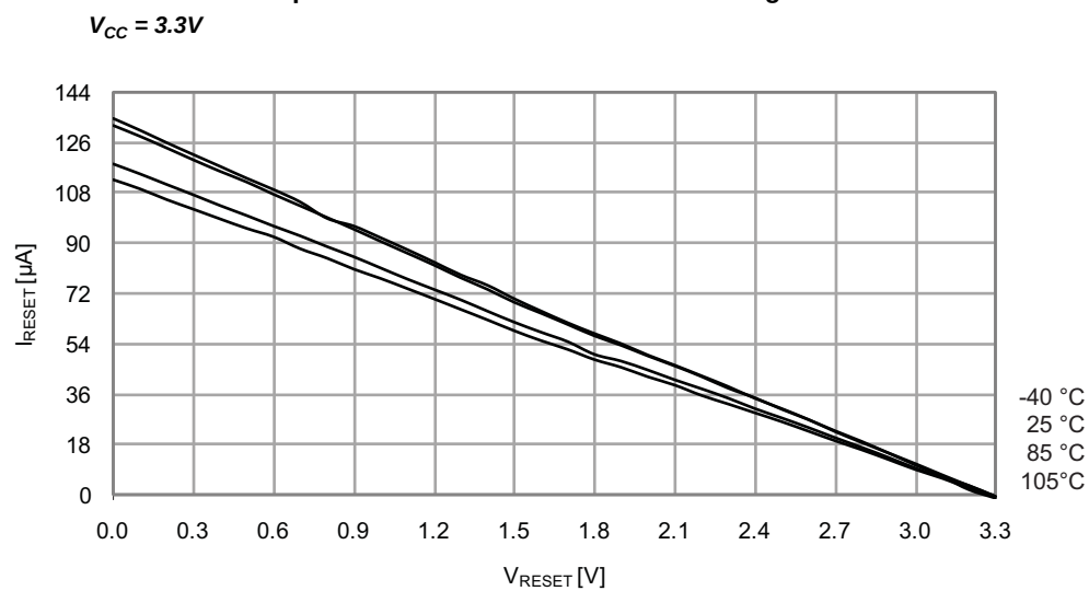
Figure 36-51. Reset Pin Pull-up Resistor Current vs. Reset Pin Voltage
