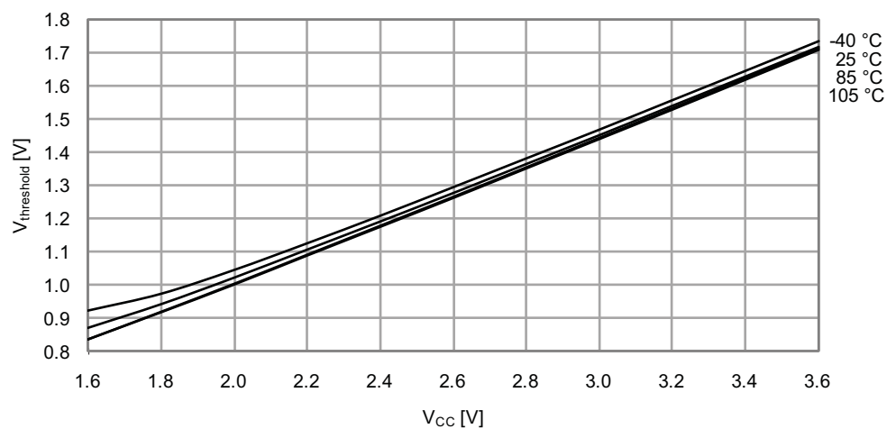
Figure 36-27. I/O Pin Input Threshold Voltage vs. V_{CC}
