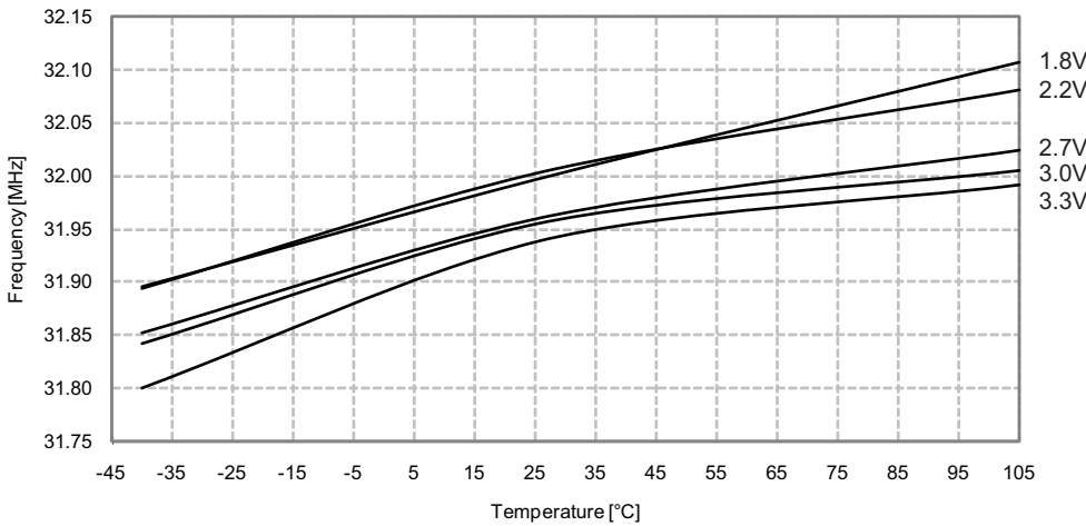
Figure 36-60. 32MHz Internal Oscillator Frequency vs. Temperature DPLL enabled, from the 32.768kHz internal oscillator
