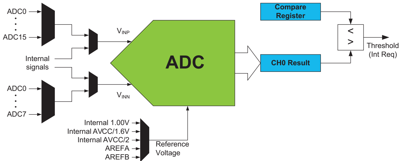
Figure 28-1. ADC Overview
