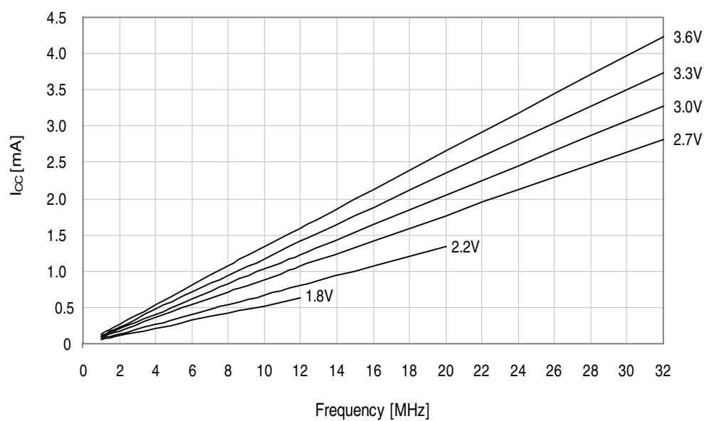
Figure 36-10. Idle Mode Supply Current vs. V_{\text{CC}}
