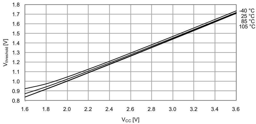
Figure 36-27. I/O Pin Input Threshold Voltage vs. V_{CC} V_{IH} I/O pin read as "1"
