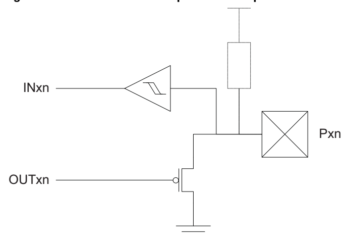
Figure 15-6. I/O Configuration - Wired-AND with Optional Pull-up
