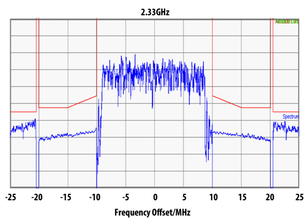
Figure 33. Spectrum Emission Mask 29.0dBm @ 2.33GHz
