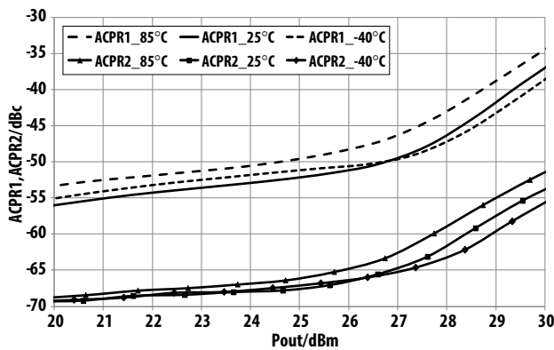
Figure 18. Over-temperature ACPR1, ACPR2 vs. P_{out} @ 2.35 GHz V_{dd}=V_{ddBias}=5.0\text{ V} operating voltage
