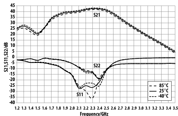
Figure 8. Small-signal performance Over-temperature V_{dd}=V_{ddBias}=5.0 V operating voltage
