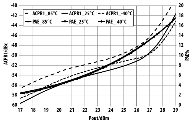
Figure 11. Over-temperature ACPR1, PAE vs. P_{out} @ 2.35 GHz V_{dd}=V_{ddBias}=5.0 V operating voltage
