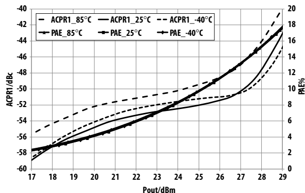
Figure 10. Over-temperature ACPR1, PAE vs. P_{out} @ 2.33 GHz V_{dd}=V_{ddBias}=5.0 V operating voltage
