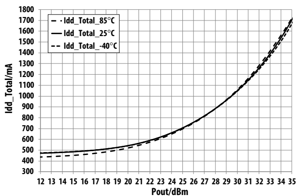
Figure 25. Over-temperature I_{dd\_total} vs. P_{out} @ 2.35 GHz V_{dd}=V_{ddBias}=5.5\text{ V} operating voltage
