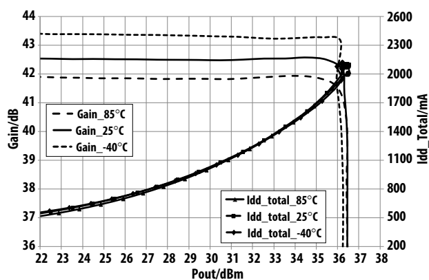
Figure 20. Over-temperature Gain, I_{dd\_total} vs. P_{out} @ 2.33GHz V_{dd}=V_{ddBias}=5.0\text{ V} operating voltage
