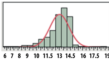
Figure 4. PAE at Pout=27.0dBm, Nominal = 13%
