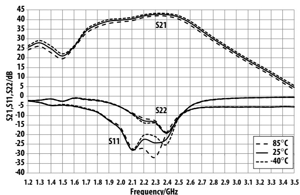
Figure 9. Small-signal performance Over-temperature V_{dd}=V_{ddBias}=5.5 V operating voltage
