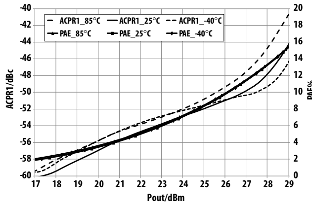
Figure 16. Over-temperature ACPR1, PAE vs. P_{out} @ 2.36 GHz V_{dd}=V_{ddBias}=5.5\text{ V} operating voltage
