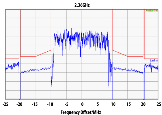
Figure 35. Spectrum Emission Mask 29.0dBm @ 2.36GHz
