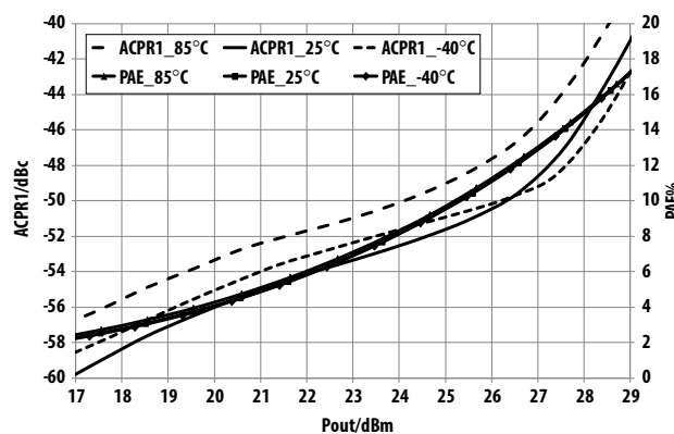
Figure 12. Over-temperature ACPR1, PAE vs. P_{out} @ 2.36 GHz V_{dd}=V_{ddBias}=5.0 V operating voltage
