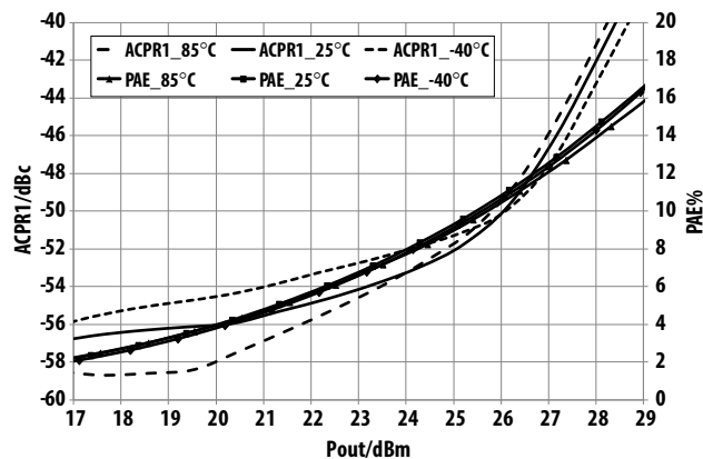
Figure 13. Over-temperature ACPR1, PAE vs. P_{out} @ 2.39 GHz V_{dd}=V_{ddBias}=5.0 V operating voltage
