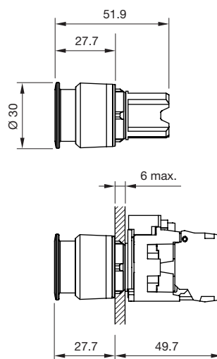
Mushroom-head pushbutton Ø 30 mm (raised design)
