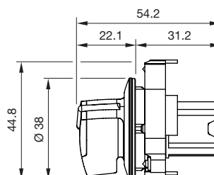
Selector switch long lever (flush design)
