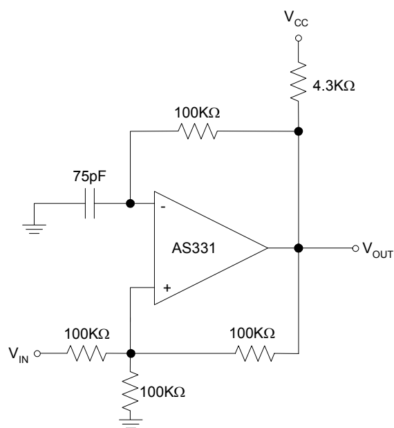
Figure 24. Squarewave Oscillator
