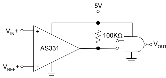
Figure 22. Driving CMOS
