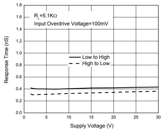
Figure 13. Response Time vs. Supply Voltage
