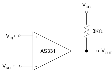
Figure 21. Basic Comparator
