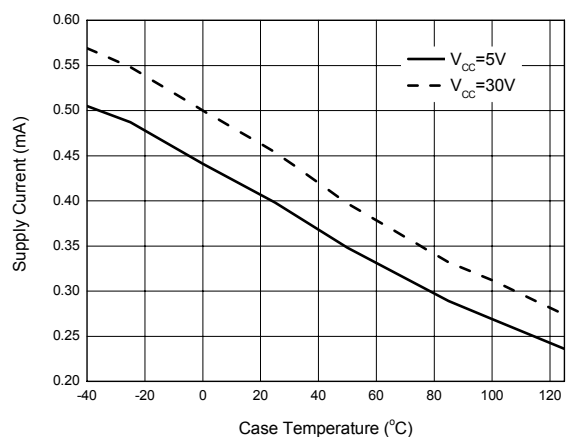
Figure 5. Supply Current vs. Case Temperature
