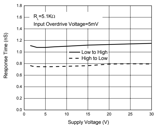
Figure 12. Response Time vs. Supply Voltage
