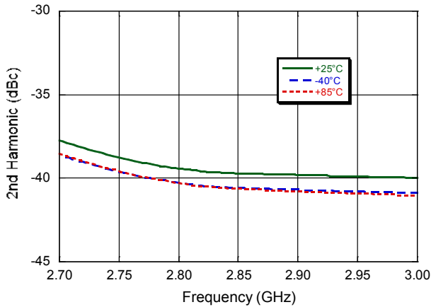
2nd Harmonic @ P3dB vs. Frequency
