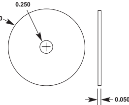
FIGURE 3. METAL COUPON
