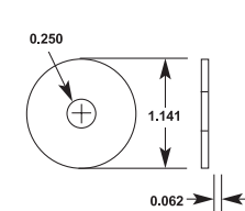
FIGURE 2. CONDUCTIVE WASHER
