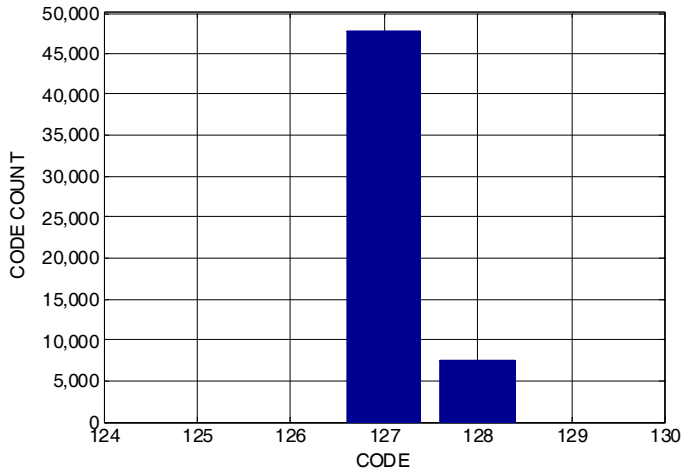
FIGURE 12. NOISE HISTOGRAM
