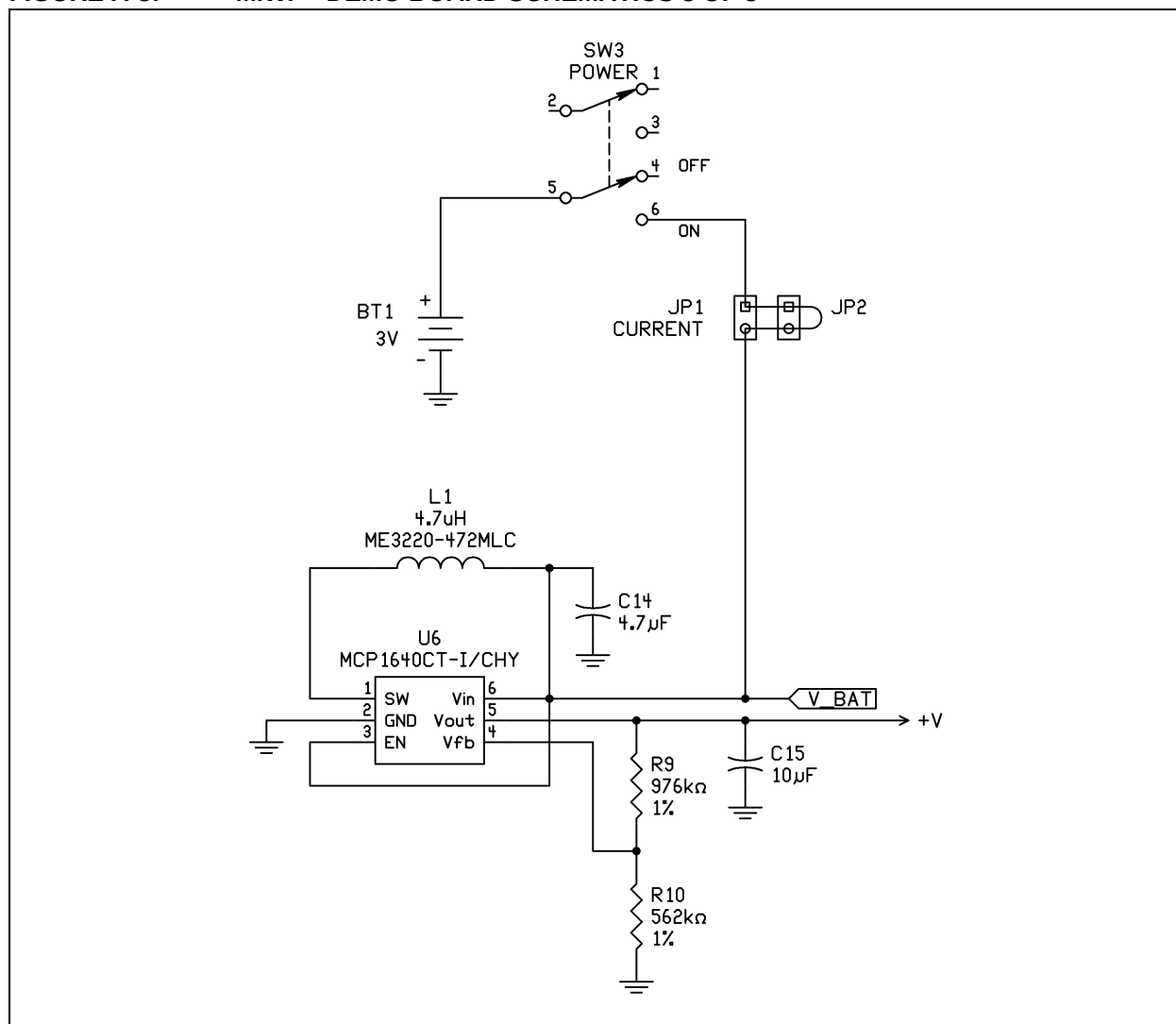
FIGURE A-3: MiWi™ DEMO BOARD SCHEMATICS 3 OF 3
