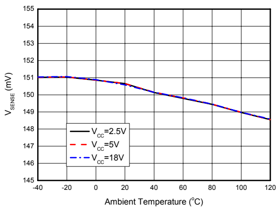
Figure 7. AP4306C V SENSE vs. Ambient Temperature
