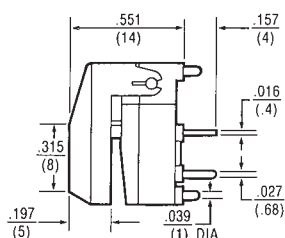
Slope Key Model
