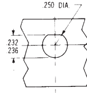
For 1/4" Flatted Bushings
