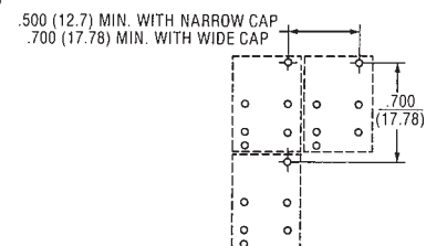
MULTIPLE SWITCH SPACING
