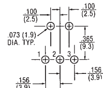
Mounting Information
