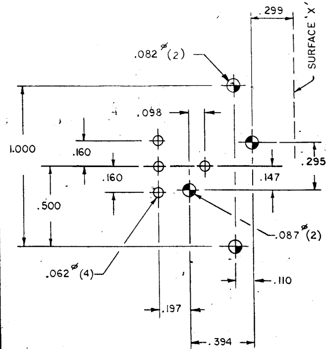
COMPONENT SIDE.
