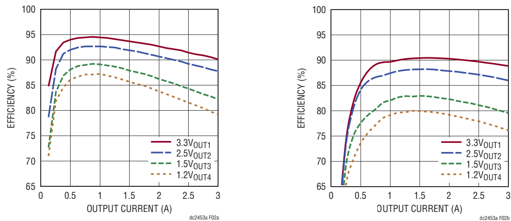
Figure 2. Measured Supply Efficiency at 5VIN and 12VIN
