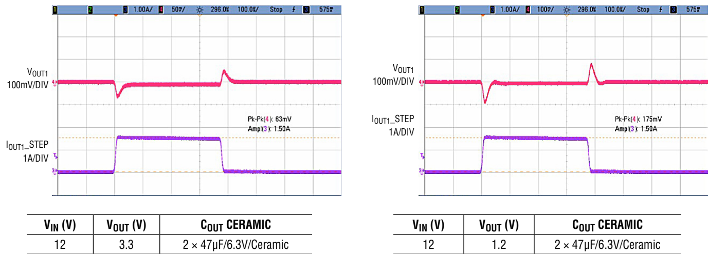
Figure 3. Measured V OUT1 = 3.3V and V OUT4 = 1.2V Load Transient Responses (1.5A to 3A Load Step)
