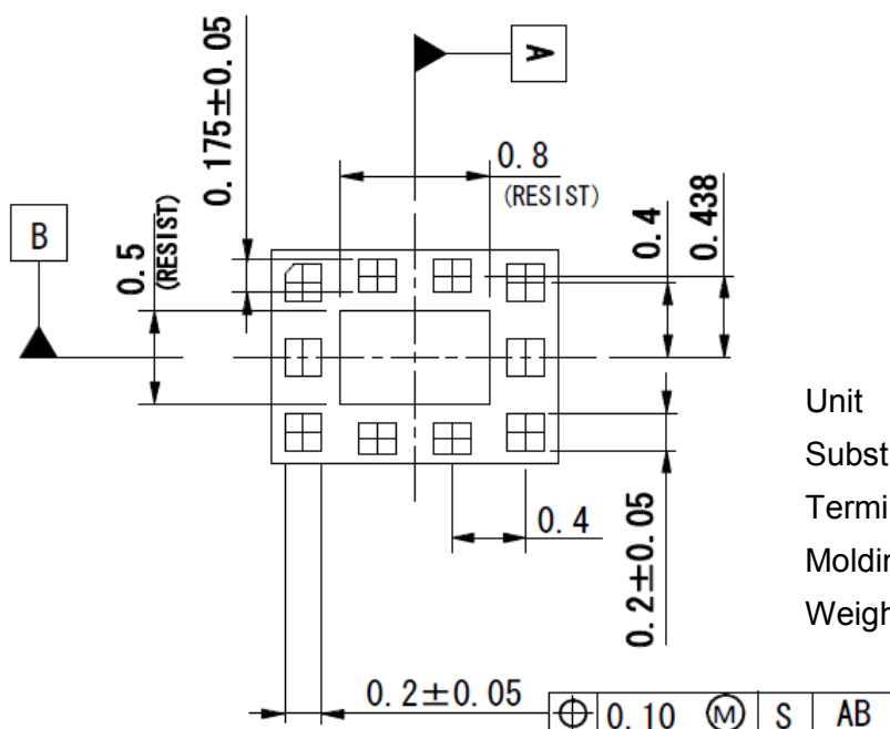
BOTTOM VIEW
