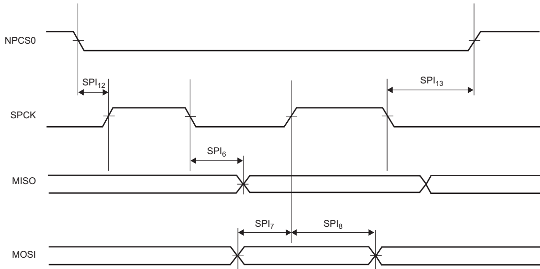
Figure 66-22. SPI Slave Modes 1 and 2
