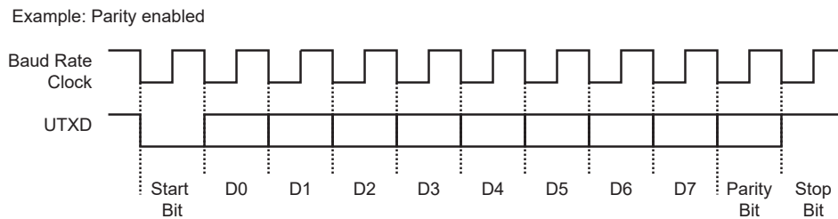
Figure 47-10. Character Transmission
