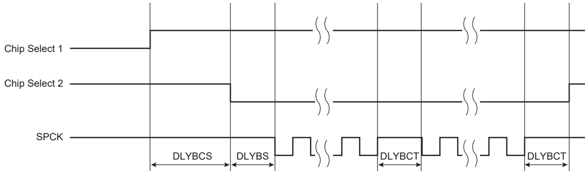
Figure 48-9. Programmable Delays
