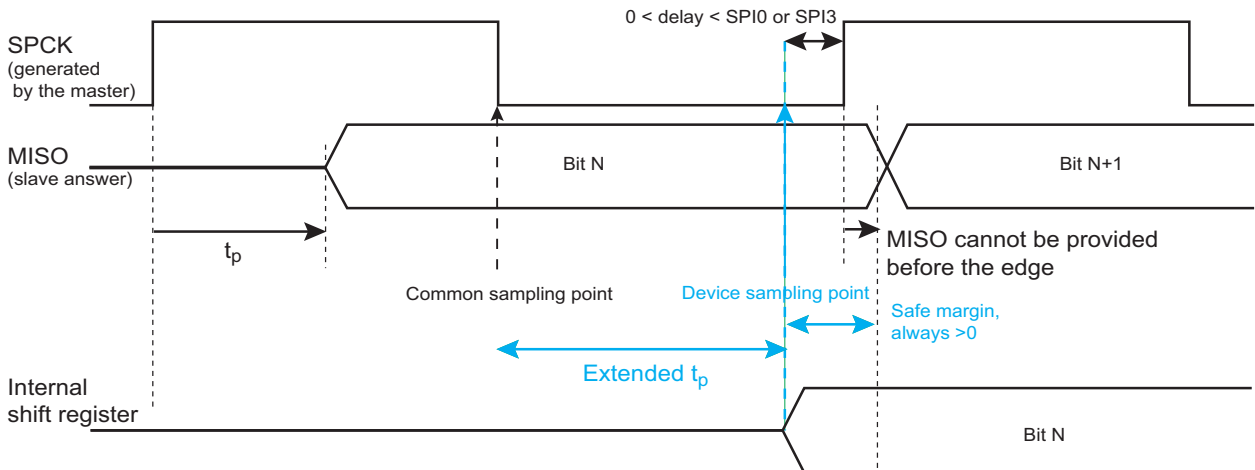
Figure 66-19. SPI Master Modes 1 and 2
