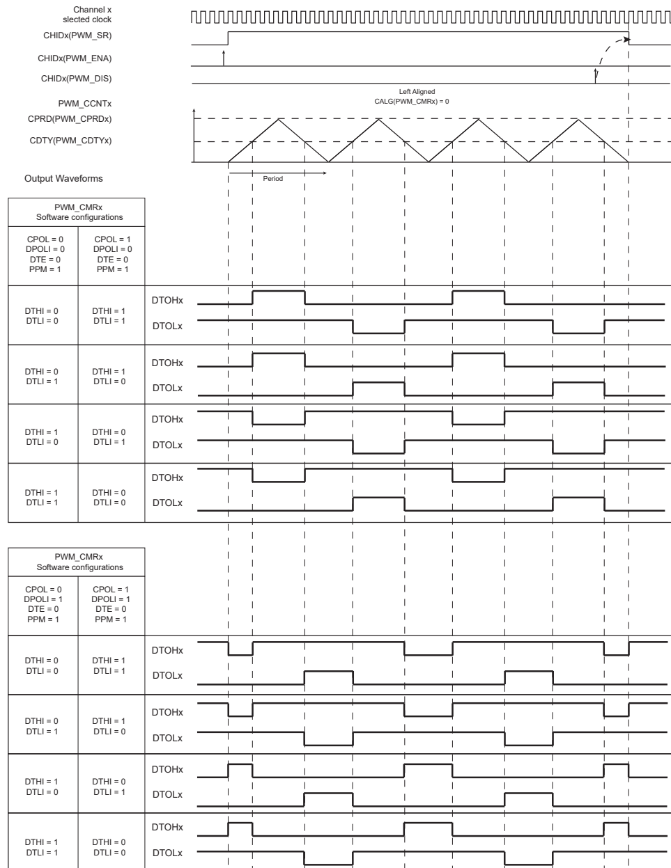
Figure 55-12. PWM Push-Pull Waveforms: Center-Aligned Mode
