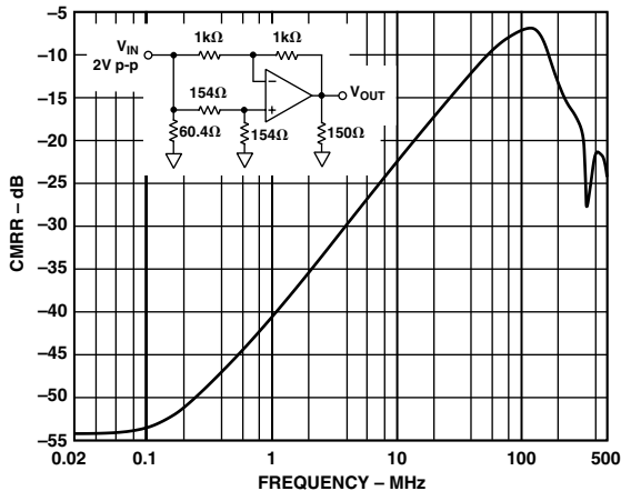
TPC 17. CMRR vs. Frequency; V_S = \pm 5\text{ V}
