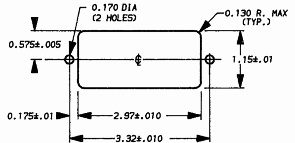
RECOMMENDED PANEL CUT-OUT NOT TO SCALE
