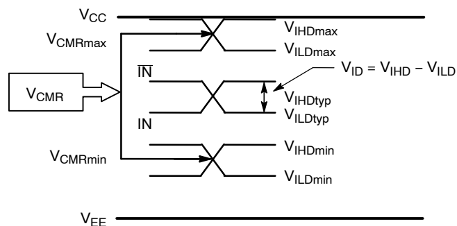
Figure 5. V_{th} Diagram
