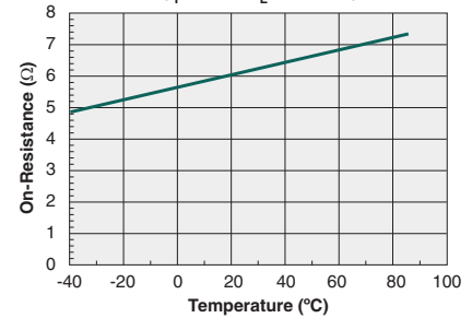
Typical On-Resistance vs. Temperature ( I_F=5\text{mA} , I_L=200\text{mA} )
