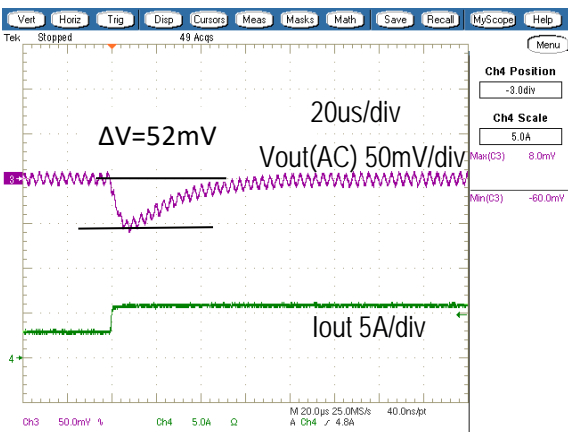
Step Load Transient Response (Vin=12V, Vout=3.3V, Cload=400uF, Iout=3A to 6A, 2.5A/us)
