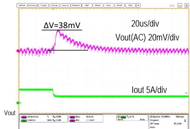
Step Load Transient Response (Vin=5.0V, Vout=1.8V, Cload=400uF, Iout=6A to 3A, 2.5A/us)
