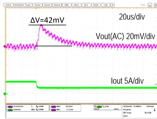
Step Load Transient Response (Vin=5.0V, Vout=0.7V, Cload=400uF, Iout=6A to 3A, 2.5A/us)
