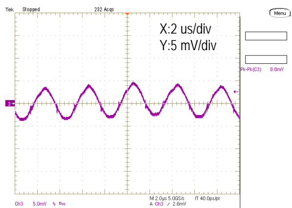
Output Ripple and Noise (Vin=5.0V, Vout=1.8V, Iout=6A, Cload=400uF, ScopeBW=20MHz)
