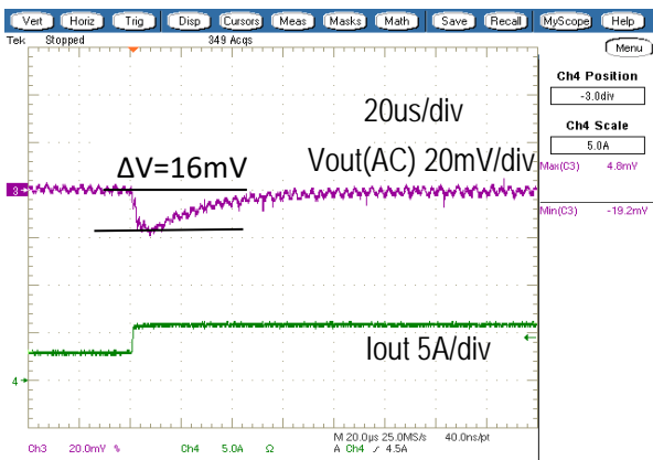
Step Load Transient Response (Vin=12V, Vout=1.0V, Cload=400uF, Iout=3A to 6A, 2.5A/us)
