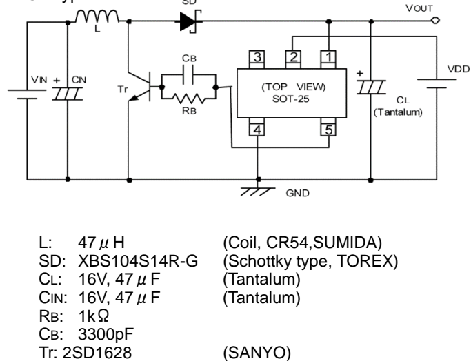
●F type circuit
