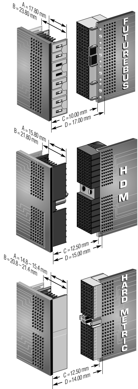
ERmet 2mm H.M. Connectors
