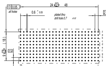
Board hole pattern (Component mounting side)
