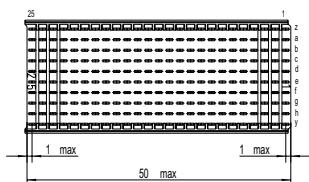
Board hole pattern (Component mounting side)
