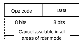
Figure 45. RDSR cancel valid timing
