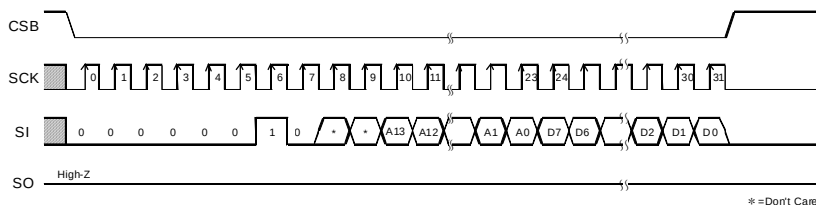
Figure 40. Write command
