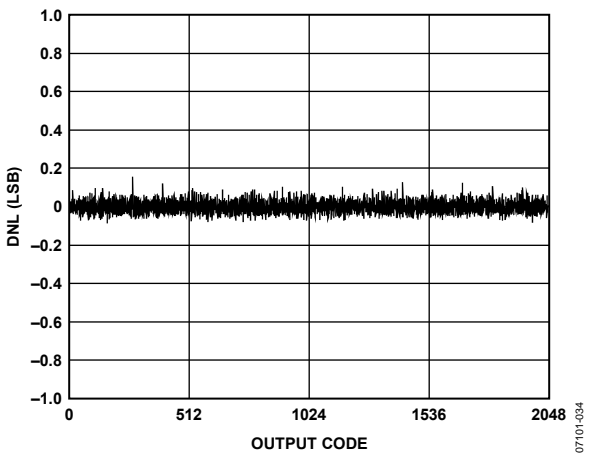
Figure 12. DNL
