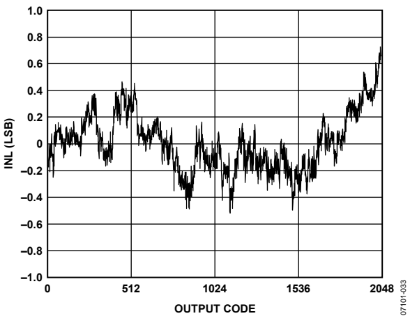
Figure 14. INL
