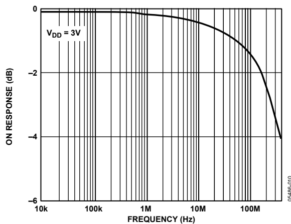
Figure 11. Bandwidth
