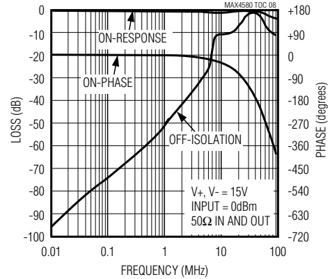
FREQUENCY RESPONSE
