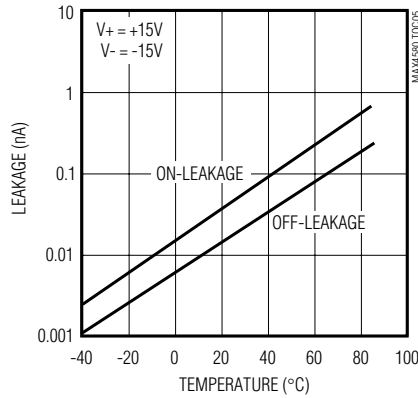
ON/OFF-LEAKAGE vs. TEMPERATURE
