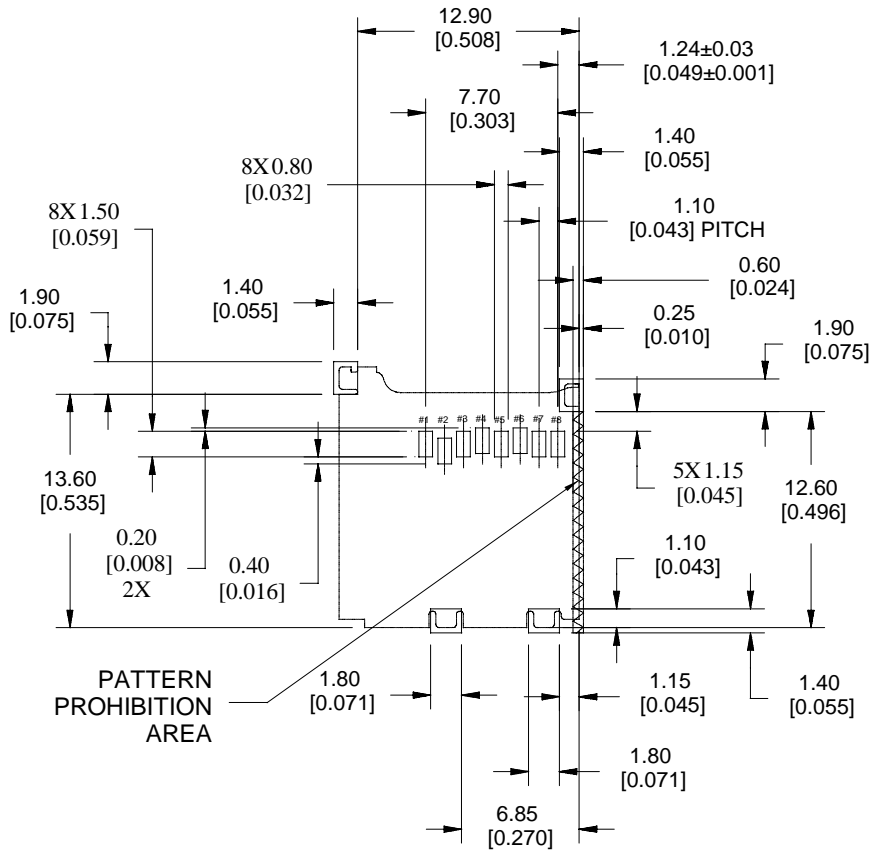
RECOMMENDED PCB PATTERN LAYOUT ± 0.05 [0.002]
