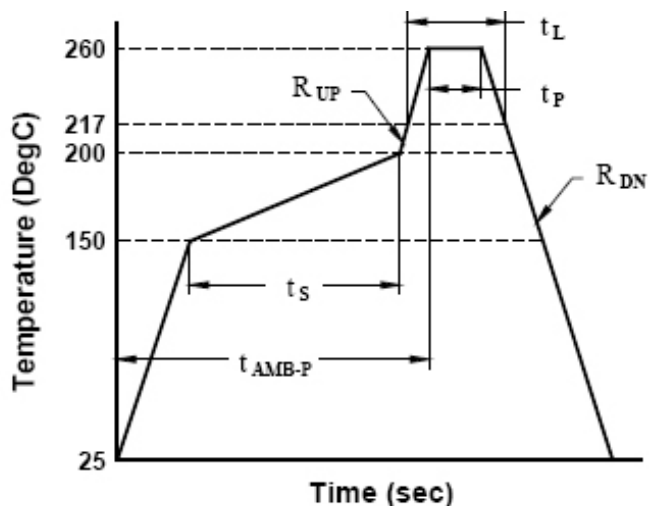
Figure 12. Suggested IR Profile
